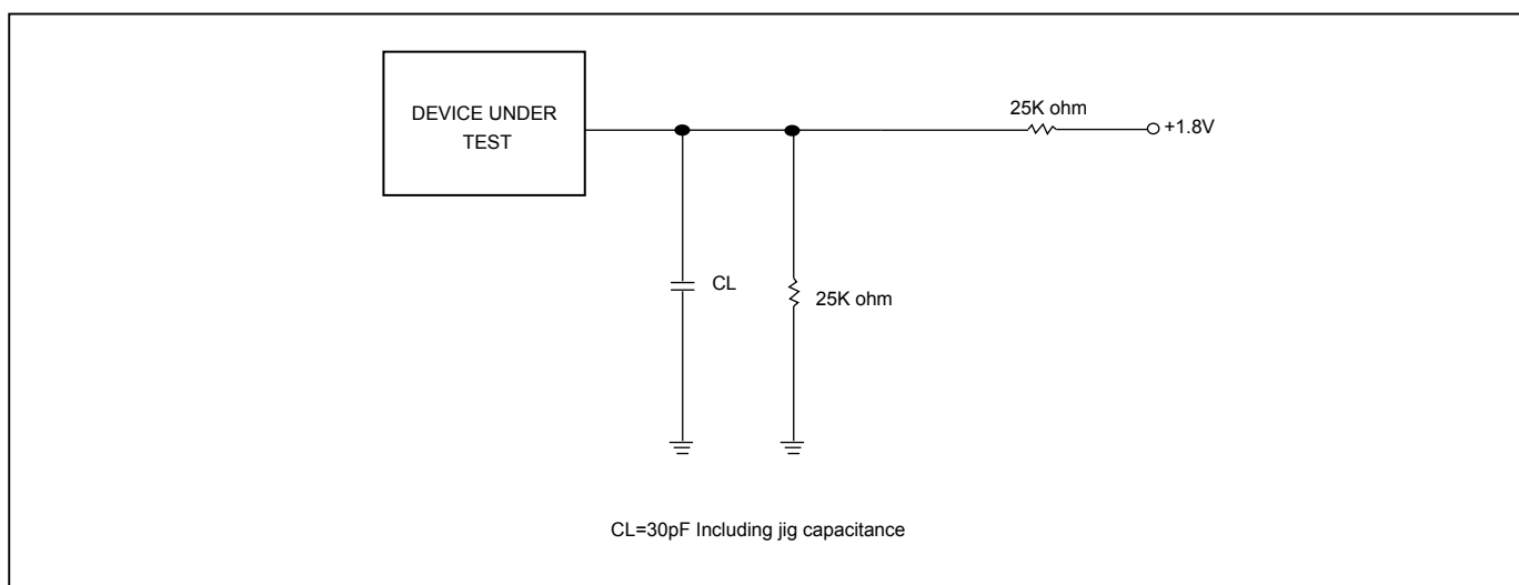
Figure 82. OUTPUT LOADING
