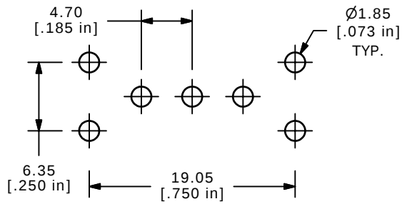
P.C. MOUNTING
