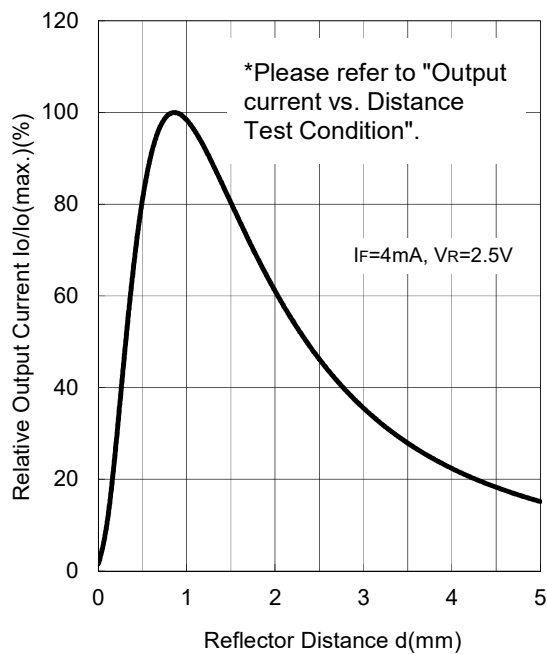
Output Current vs. Distance RED LED ( T_a=25^\circ\text{C} )
