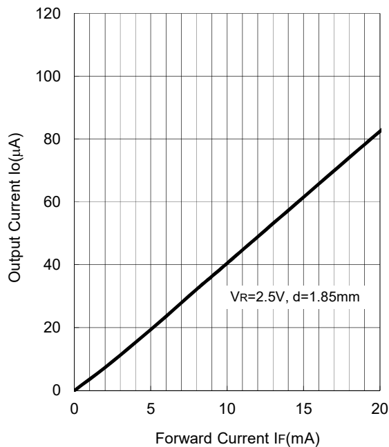
Output Current vs. Forward Current RED LED ( T_a=25^\circ\text{C} )
