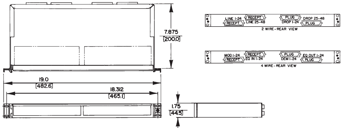
2- & 4-Wire Connectorized Jackfields (4-Wire Style Shown)
