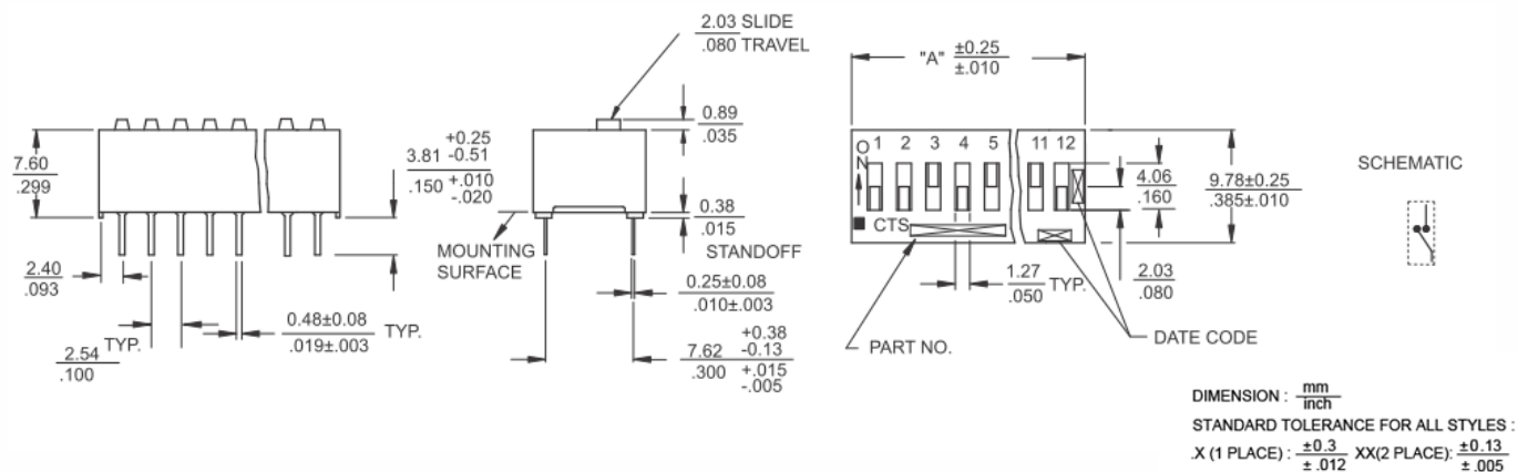
Figure 1 - SPST
