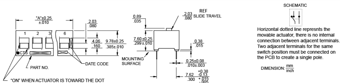
Figure 2 – SPDT
