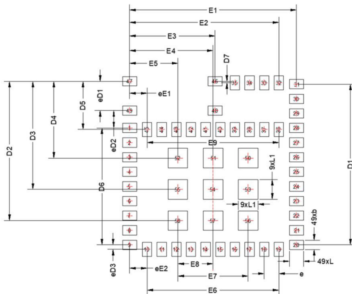
Figure 8.1. WFM200S Land Pattern
