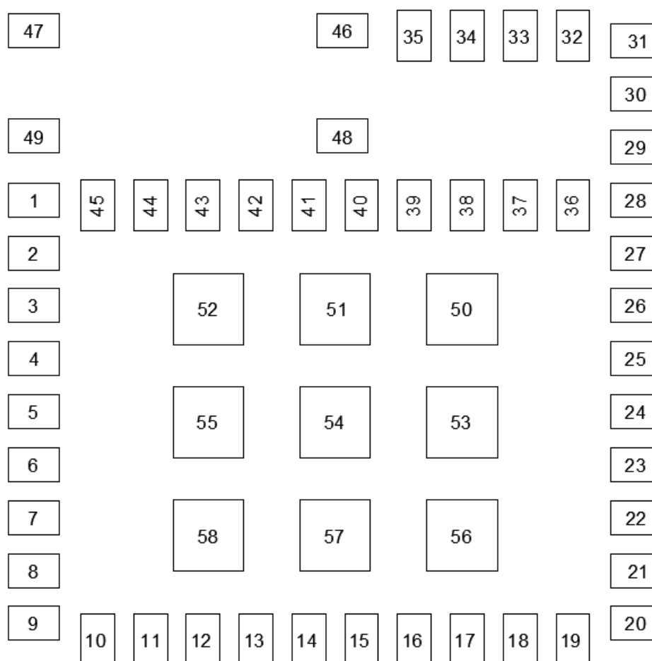
Figure 6.1. WFM200S Pinout
