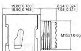
Rear output #2 Accessory Thread
