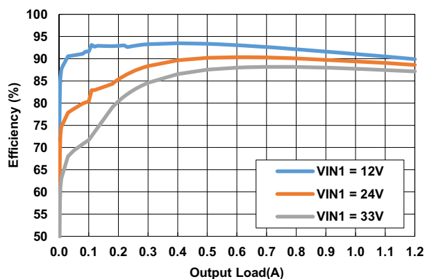
Figure 2. Efficiency vs Load, PFM, V_{OUT} = 5\text{V} , L_1 = 22\mu\text{H}
