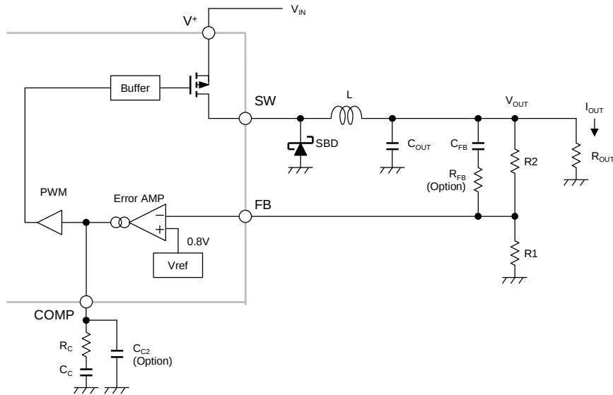
Fig. 7. Compensation Circuit Configuration
