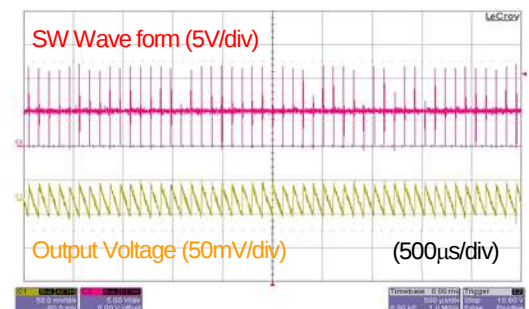
b) Waveform of I_{OUT}=10mA
