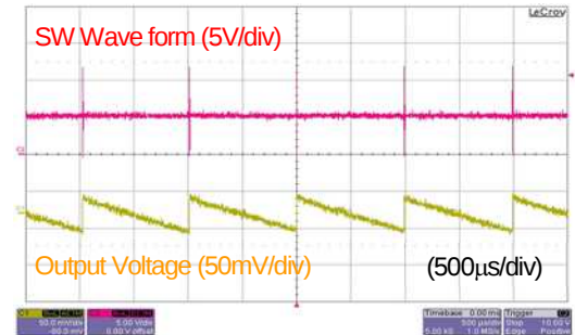
a) Waveform of I_{OUT}=1mA
