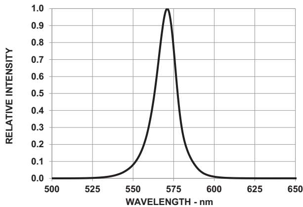
Figure 11: Relative Intensity vs. Wavelength
