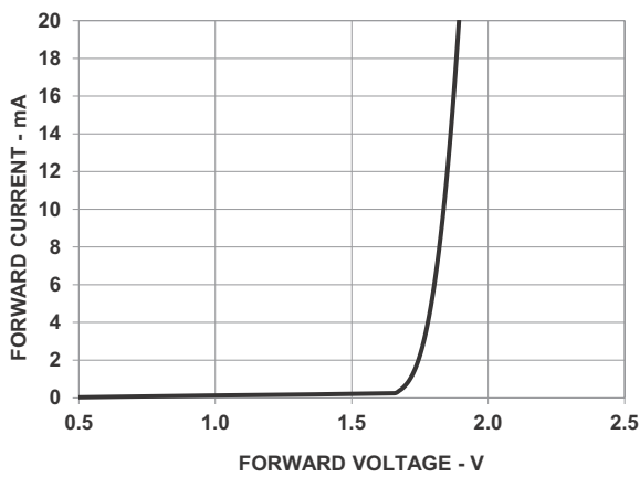
Figure 8: Forward Current vs. Forward Voltage
