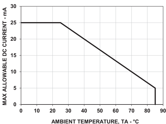
Figure 14: Maximum Forward Current vs. Ambient Temperature
