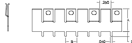
FIGURE 6 .25" Pin Spacing, No Standoff
