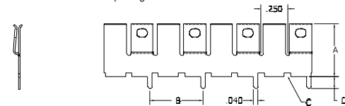
FIGURE 2 .50" Pin Spacing
