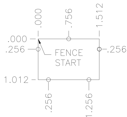
1.0" Pin Pattern
