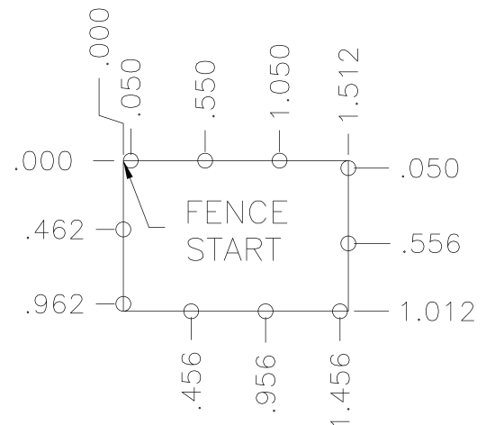
.50" Pin Pattern
