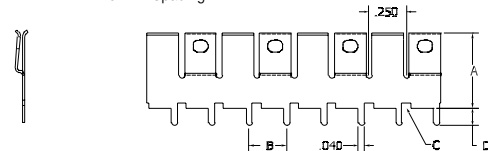
FIGURE 3 .25" Pin Spacing
