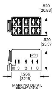
VC2 CONNECTOR HOUSING (For AMP terminals only)
