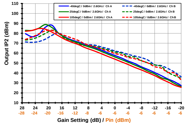
Output IP2 [2.6 GHz]
