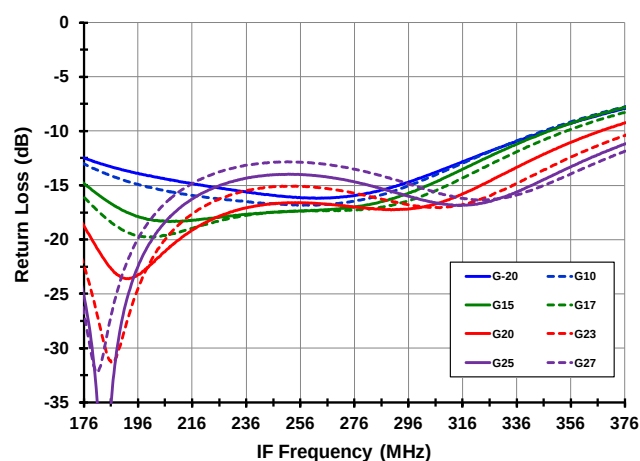
IF_B Output Return Loss 276MHz match
