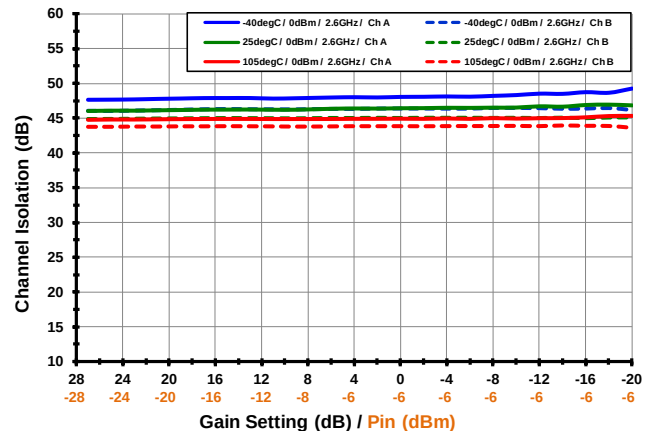
Channel Isolation [2.6 GHz]
