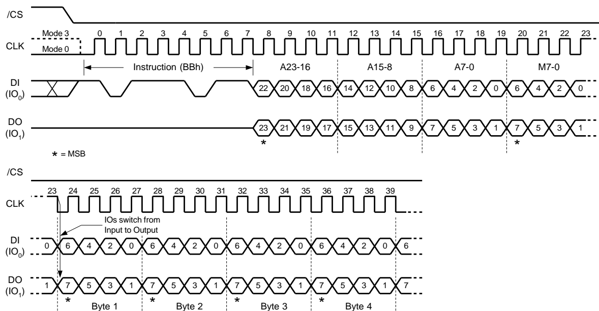
Figure 23a. Fast Read Dual I/O (Initial instruction or previous M5-4≠10, SPI Mode only)
