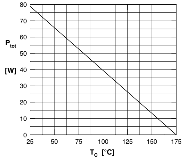
Fig. 4 Power derating
