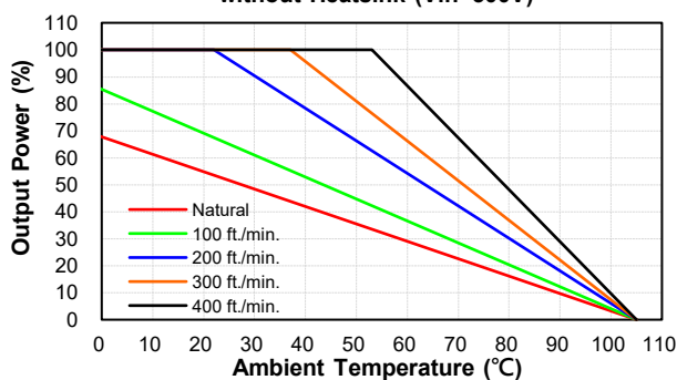
CQB75-300S3V3, 05 Derating Curve without Heatsink (Vin=300V)
