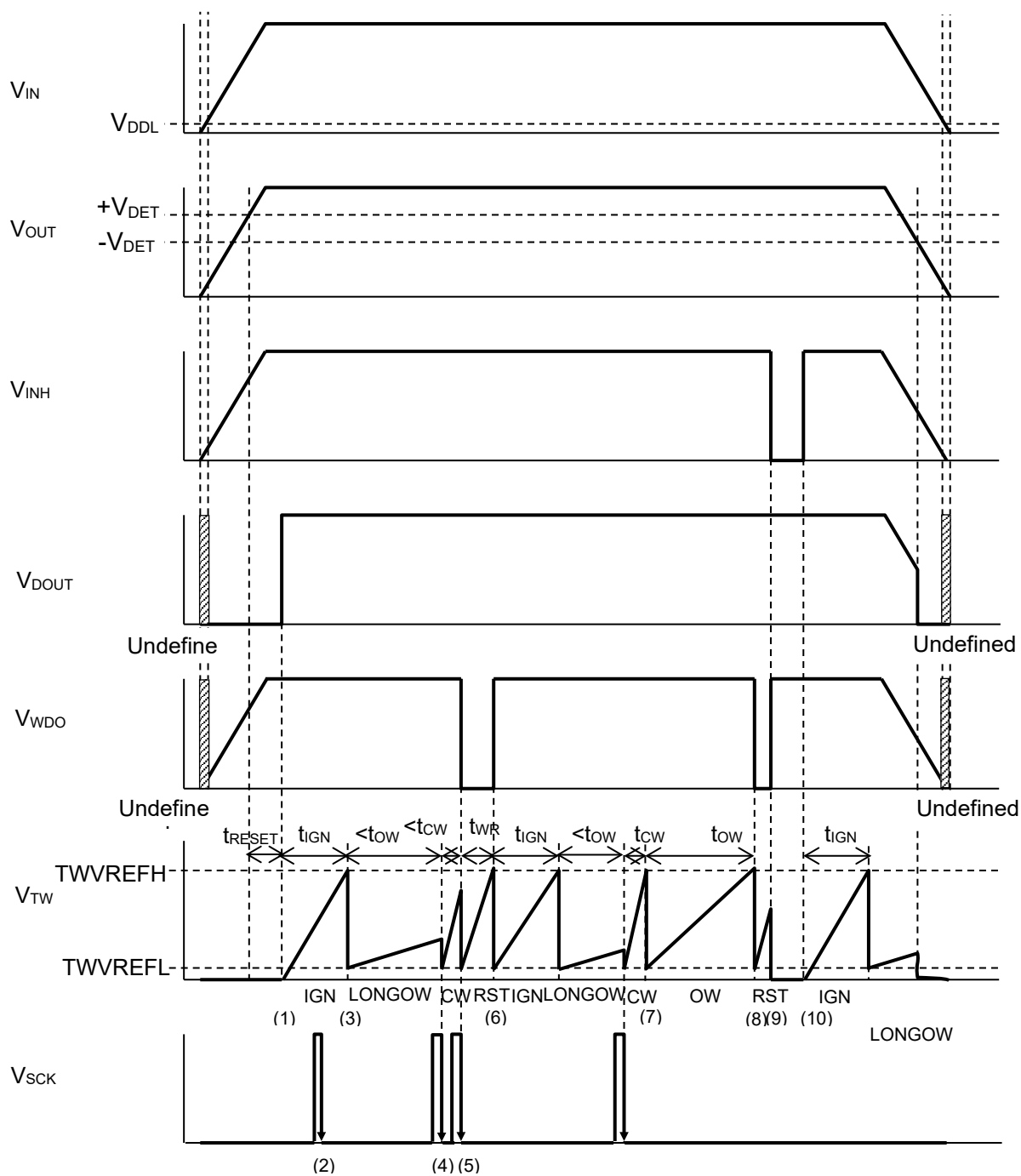
R5115xxx2C WDT Timing Chart, Window Type
