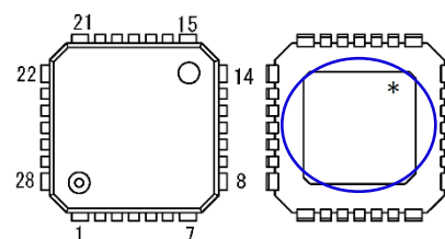
HQFN0808-28 Pin Configuration
