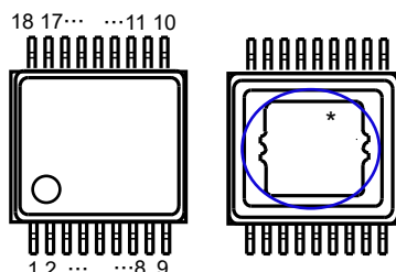
HSOP-18 Pin Configuration
