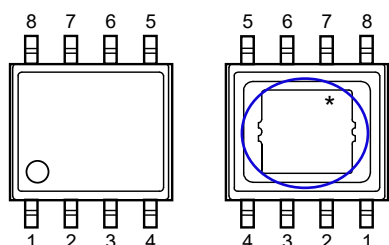
HSOP-8E Pin Configuration
