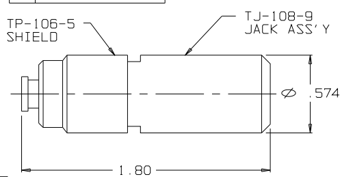
B1 TJ-108-10 JACK & SHIELD ASSEMBLY
