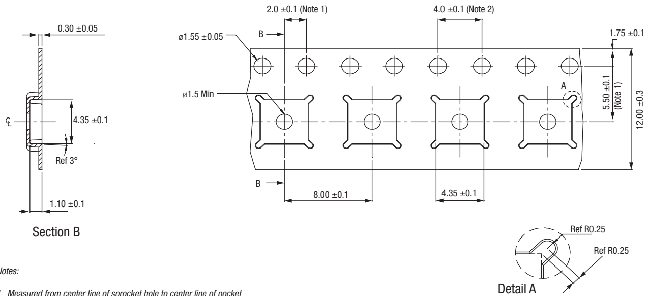
Figure 8. SKY85402-11 Tape and Reel Dimensions
