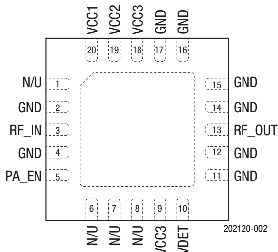
Figure 2. SKY85402-11 Pinout (Top View)
