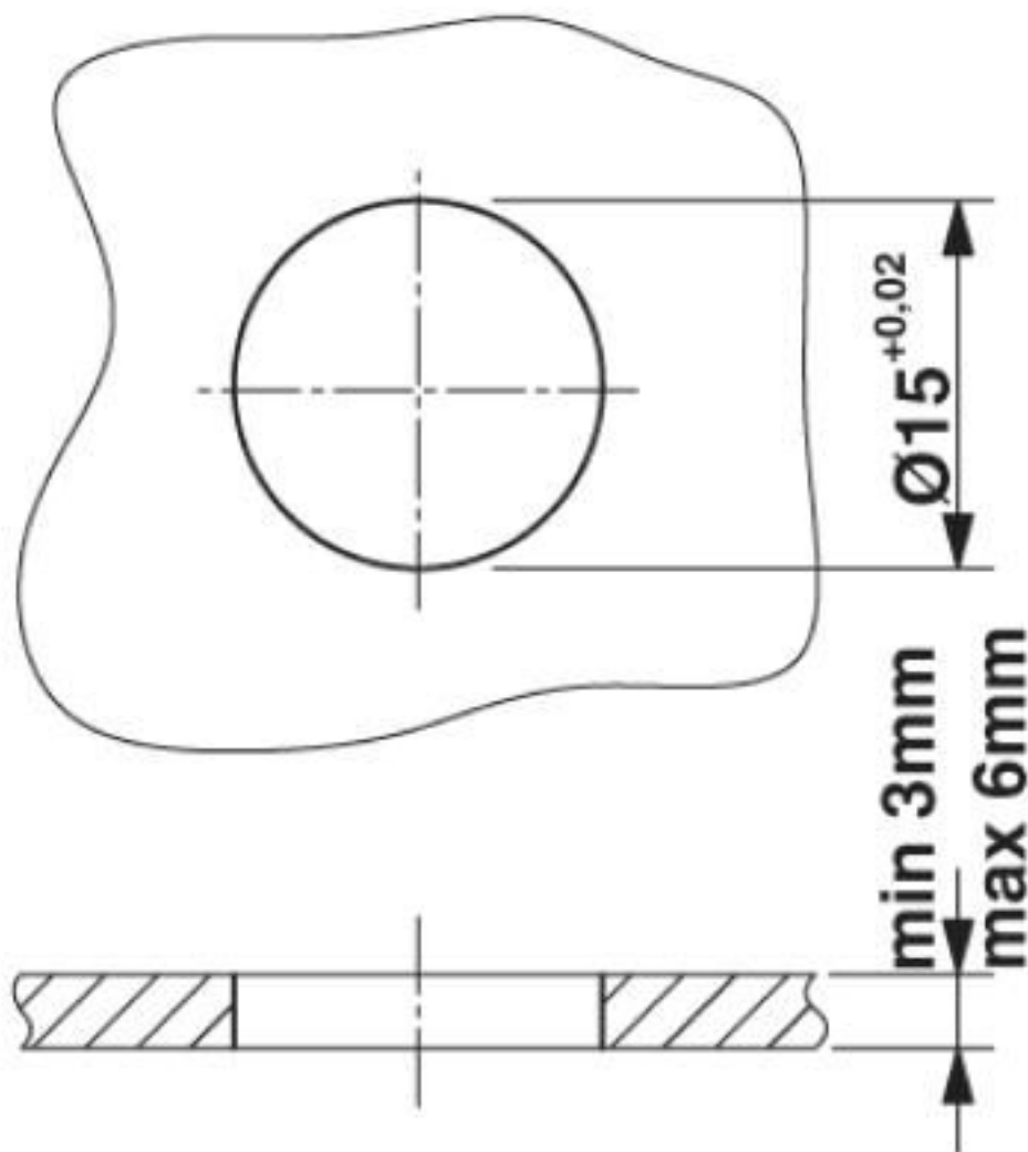
Dimensional drawing
