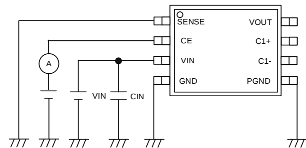
CIRCUIT⑤
