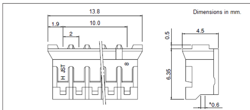
Figure 7. Receptacle Drawing
