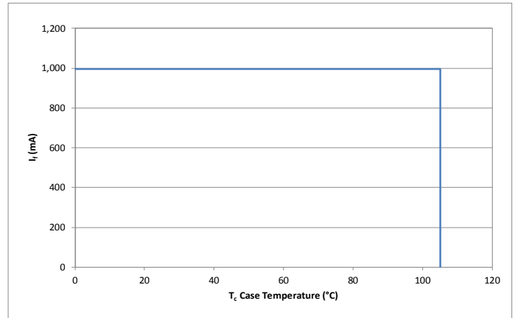
Derating Curve
