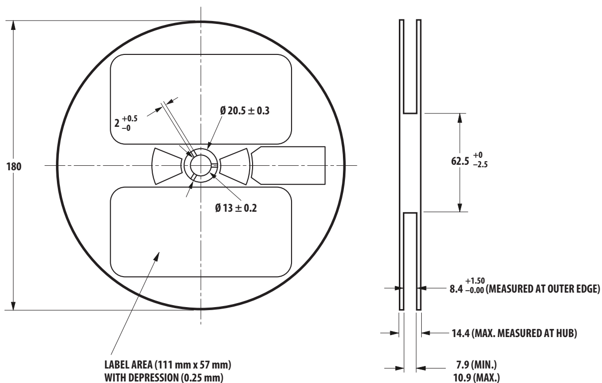
Figure 14: Reel Dimensions
