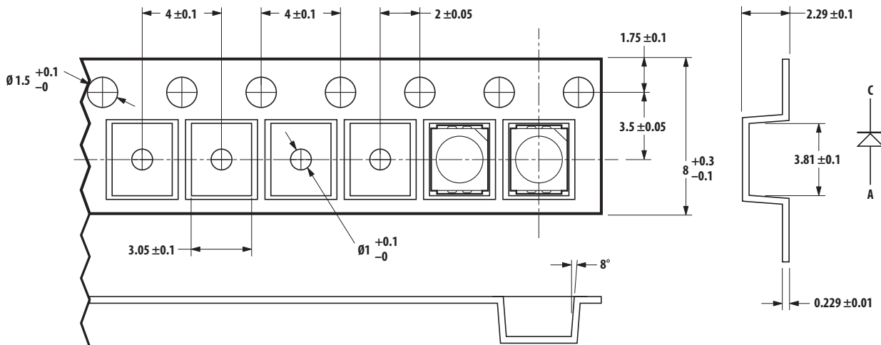
Figure 13: Tape Dimensions
