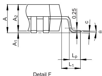
Figure D 80-Pin LQFP (PLQP0080JA-B)
