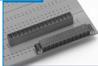
ELXH Headers Hor/Ver . . . . Page 16 ELXH with Locking Ears . . . Page 18 12A / 300V
