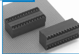
ELFA 2-Tier Aligned H/V . . . Page 38 15A / 300V
