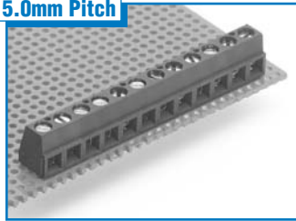
ESLM Low-Profile, R/A . . . Page 67 13.5A / 300V
