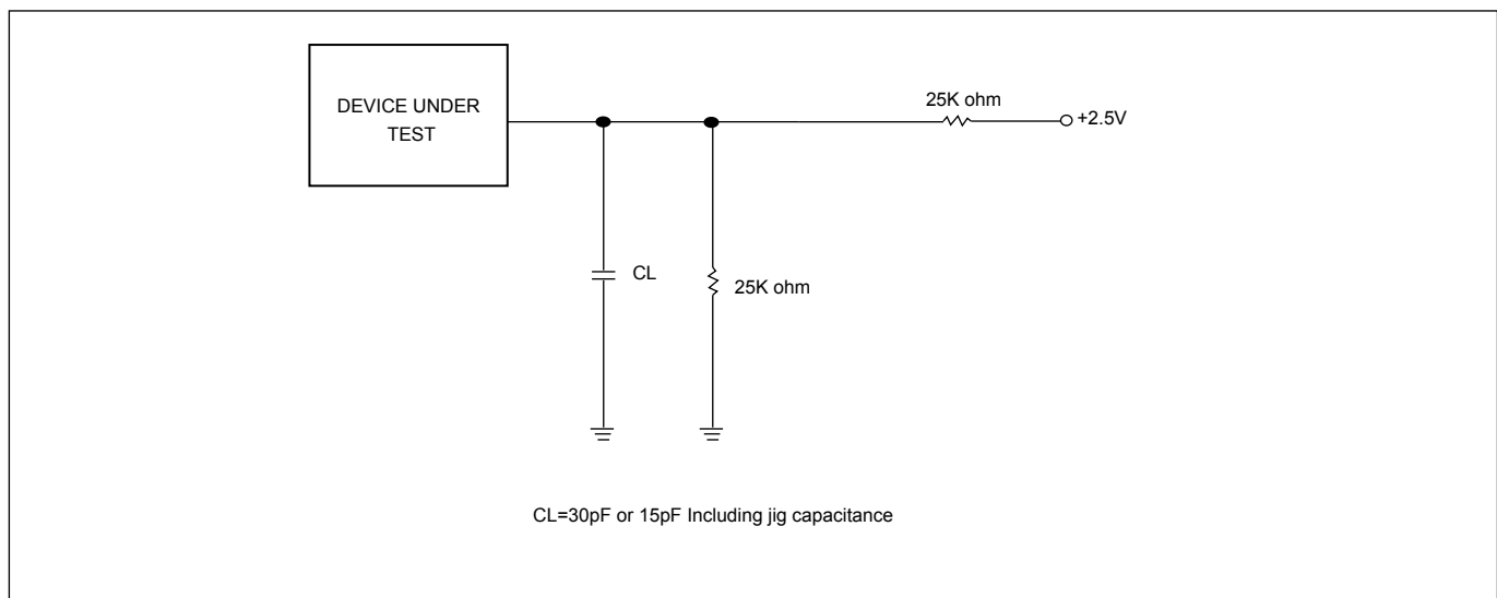
Figure 30. OUTPUT LOADING
