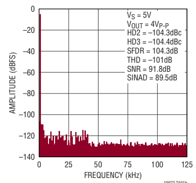
LT1997-2 Driving LTC2364-16, ADC, f_{\text{IN}} = 1\text{kHz} , 32768-Point FFT
