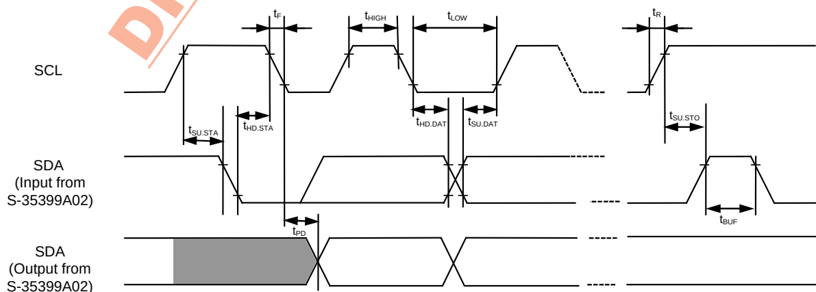
Figure 10 Bus Timing
