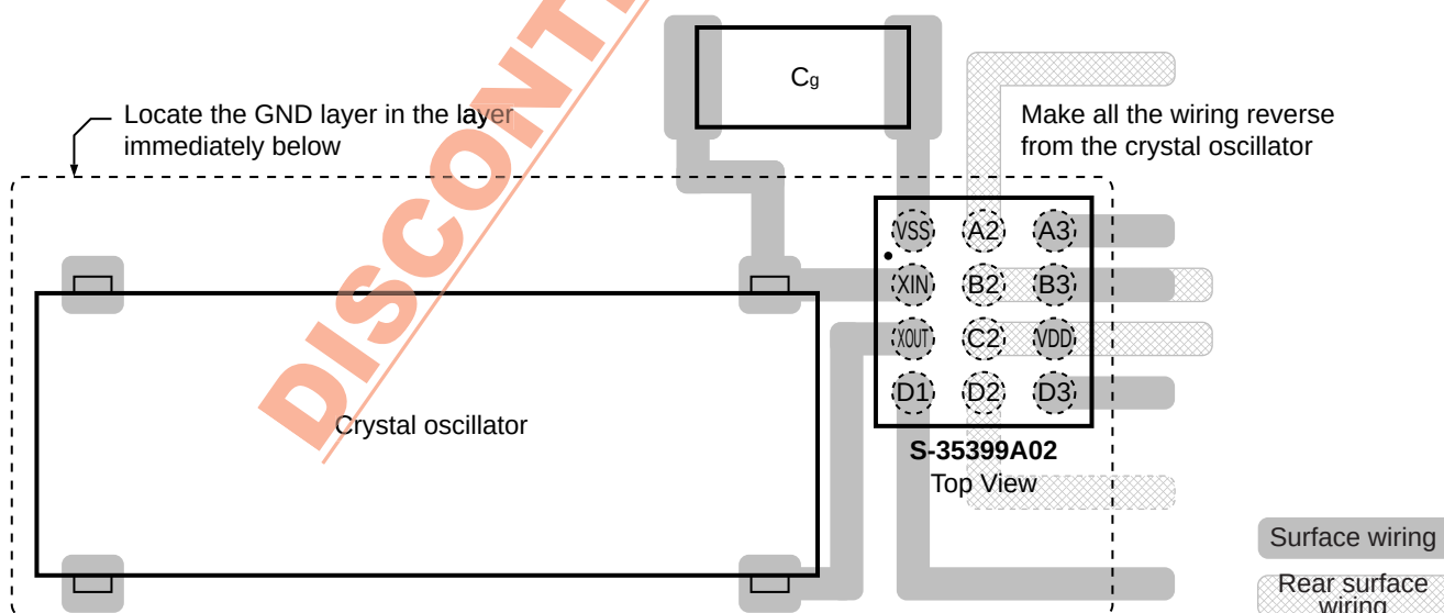
Figure 61 Connection Diagram 2
