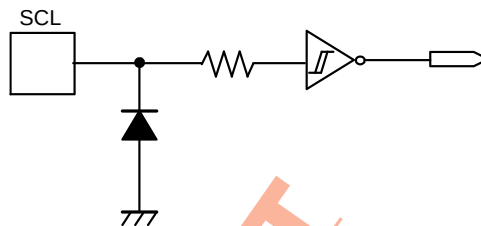
Figure 4 SCL Pin
