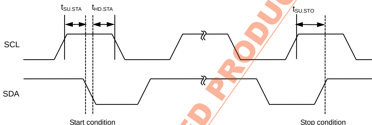
Figure 40 Start/Stop Conditions
