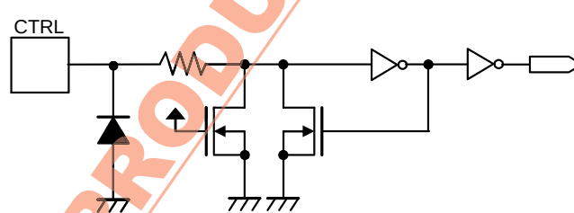
Figure 6 CTRL Pin
