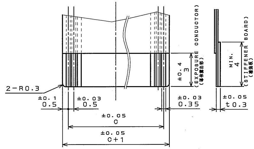
APPLICABLE F.P.C. DIMENSION(REF.) 適合FPC寸法(参考)
