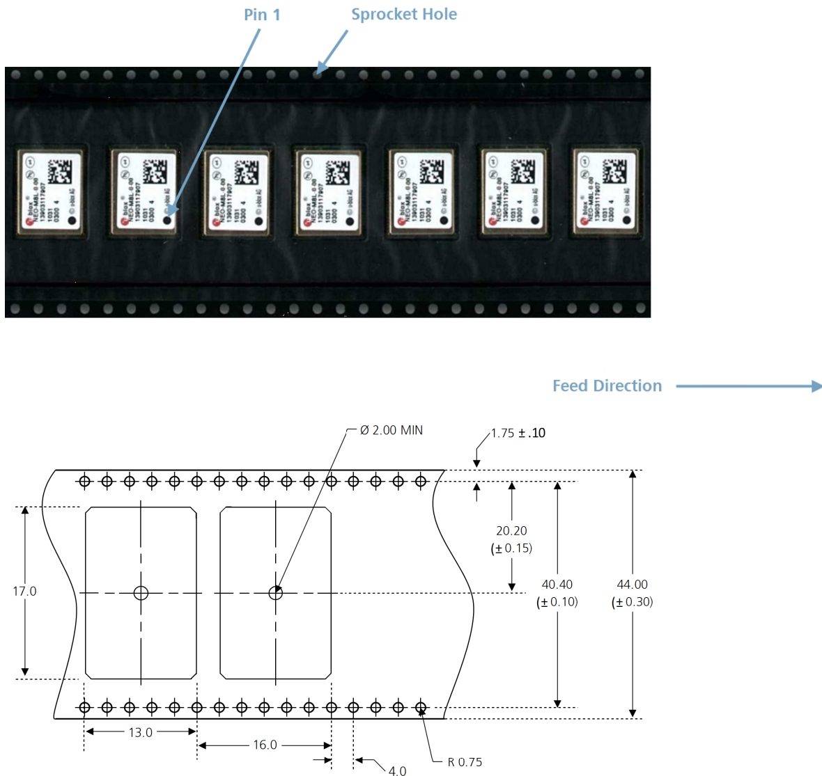
Figure 5: Dimensions and orientation for NEO-M8L-06B modules on tape
