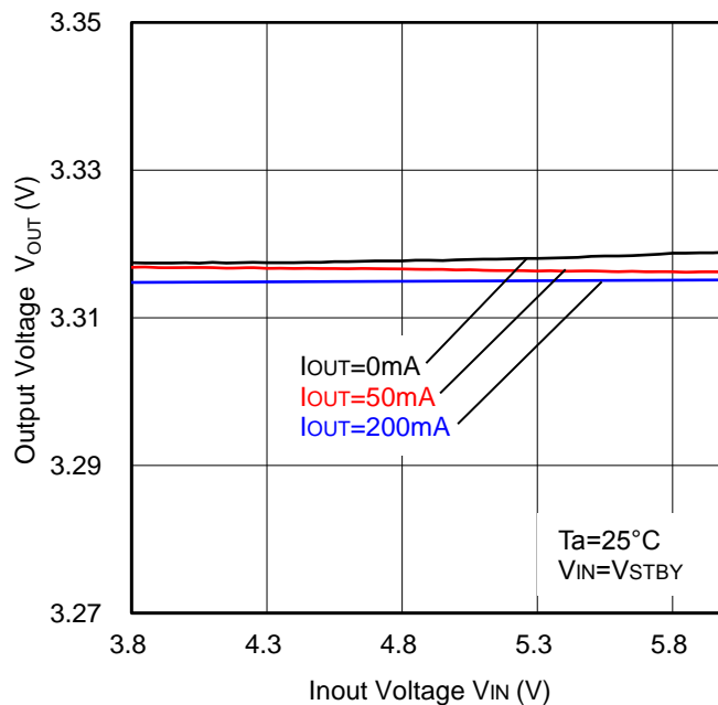
Figure 27. Line Regulation
