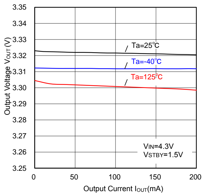
Figure 29. Load Regulation
