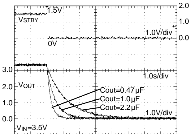
Figure 47. Discharge Time ( R_{OUT}=\text{open} )
