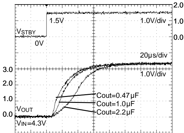
Figure 45. Startup Time ( R_{OUT}=\text{open} )
