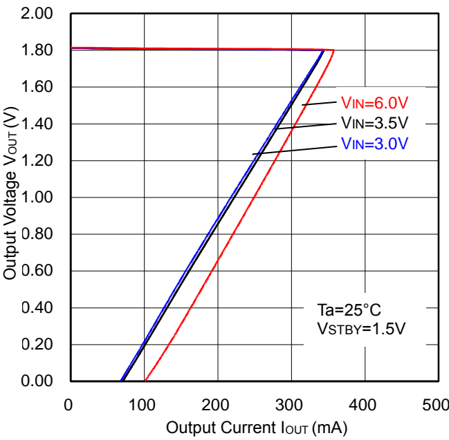
Figure 8. OCP Threshold
