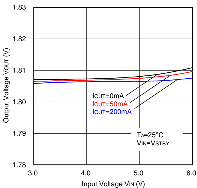
Figure 4. Line Regulation
