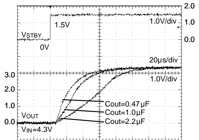
Figure 46. Startup Time ( R_{OUT}=16.5\Omega )
