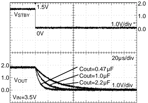
Figure 25. Discharge Time ( R_{OUT}=9\Omega )
