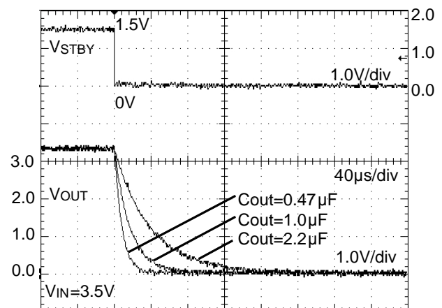
Figure 48. Discharge Time ( R_{OUT}=16.5\Omega )
