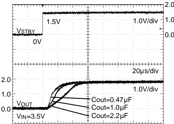
Figure 23. Startup Time ( R_{OUT}=9\Omega )
