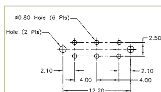
P.C. MOUNTING
