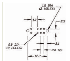
P.C. MOUNTING
