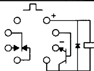
TERMINAL VIEW
