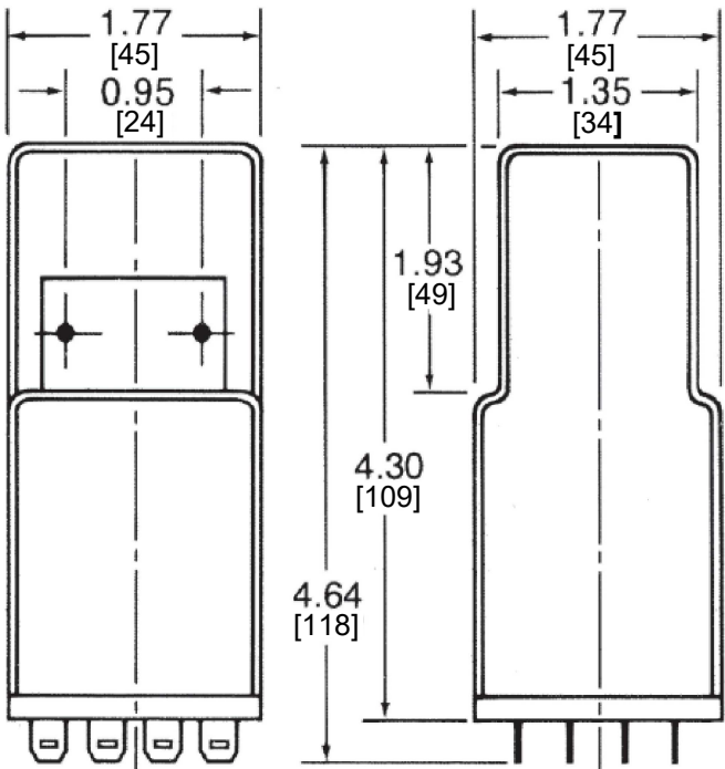
Outline Dimensions
