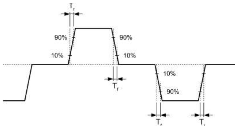
Figure 5-3 - 100Base-TX T_{r/f} Timing
