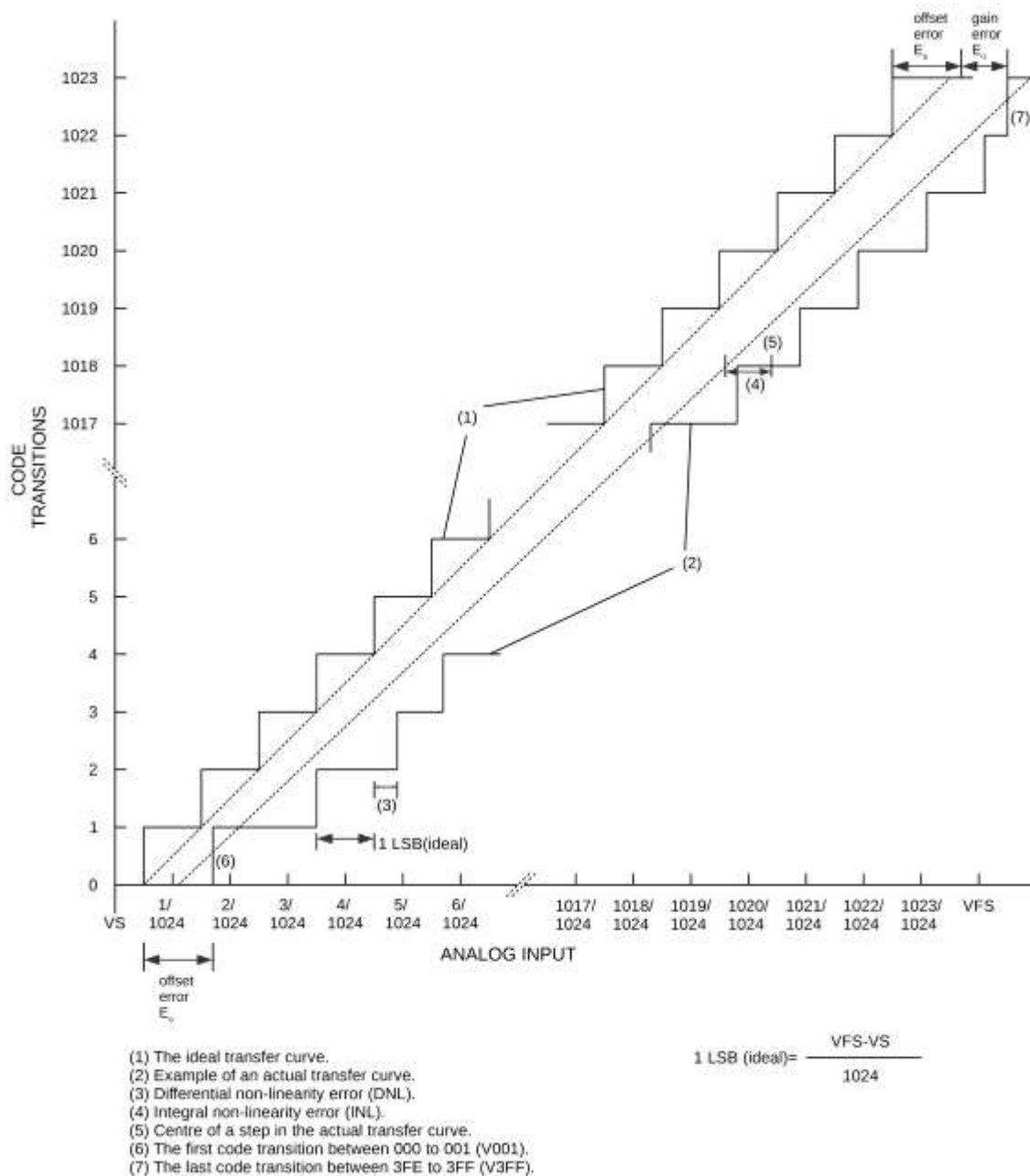
Figure 5-1 ADC Characteristics
