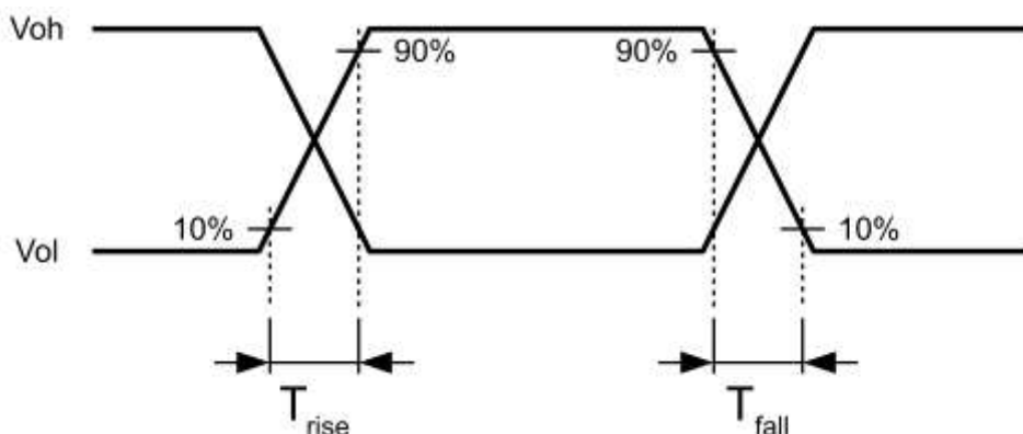
Figure 5-2 - USB Rise and Fall Times for DP/DM
