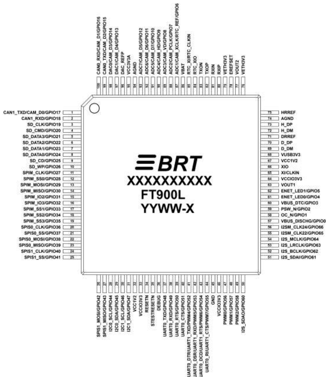
Figure 3-5 - Pin Configuration FT900L (top-down view)
