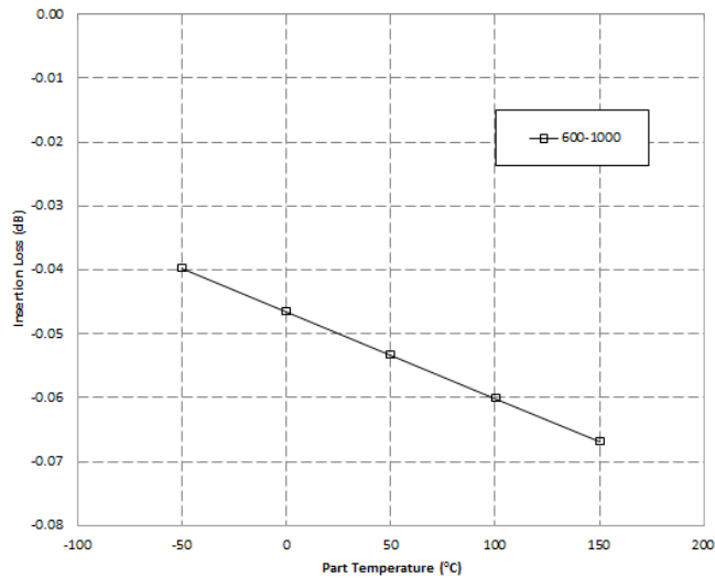
X4C09F1-30S Typical Insertion Loss Derating Curve
