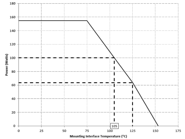
X4C09F1-30S Power Derating Curve
