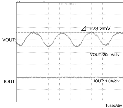
Fig.16 Output Ripple Voltage ( V_{IN} = 12V V_{OUT} = 3.3V L = 10\mu H C_{out} = 22\mu F I_{out} = 2.0A )
