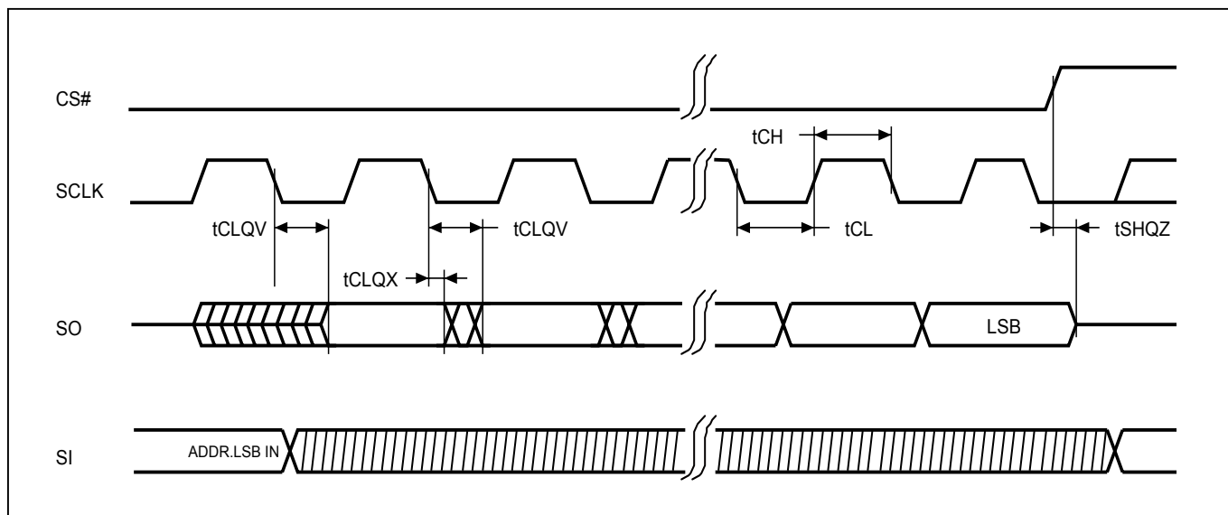
Figure 7. Output Timing
