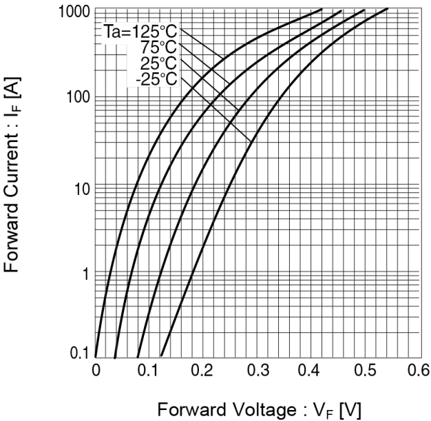
Fig.11 Forward Current vs. Forward Voltage
