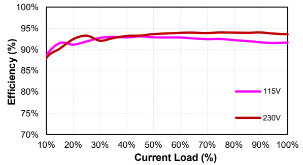
CFM500M180 (Eff Vs Io)
