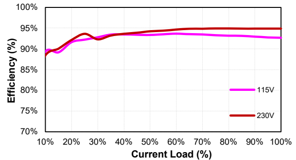
CFM500M360 (Eff Vs Io)
