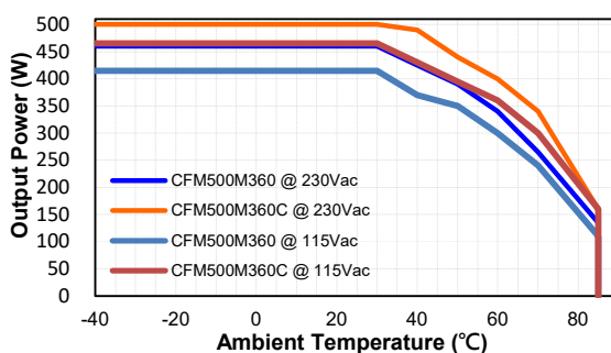
Output power vs Ambient Temperature
