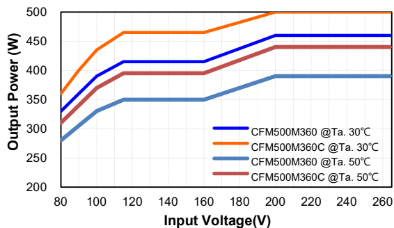
Output power & Input Voltage
