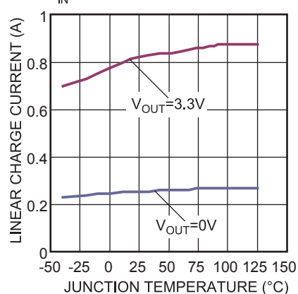
Linear Charge Current vs. Junction Temperature V_{IN} = 4.2V
