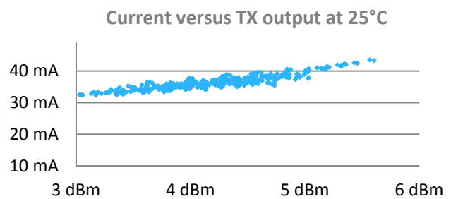
Figure 4: Typical current consumption versus TX power
