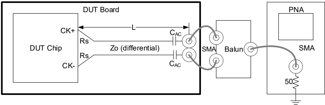
Figure 8. Test Setup for PCIe Clock Phase Jitter Measurements
