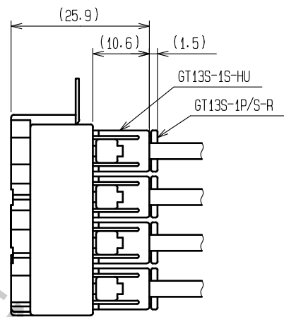
MATED CONNECTOR
