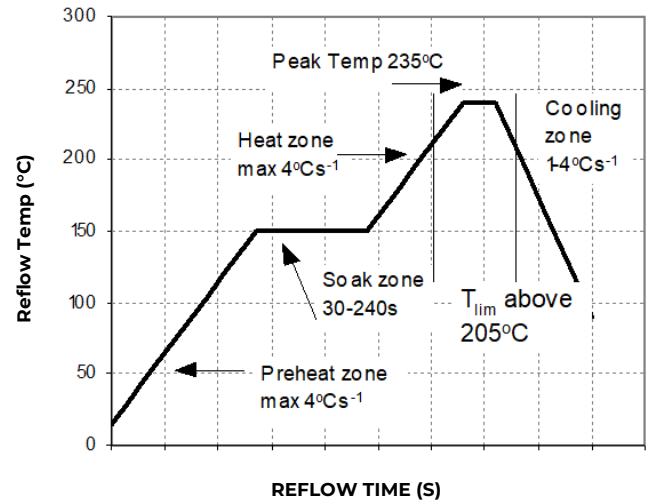
Figure 21. Reflow Profile for Tin/Lead (Sn/Pb) process.
