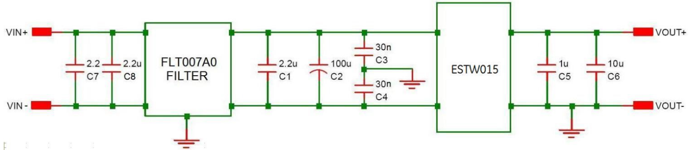
Figure 24. EMC Considerations
