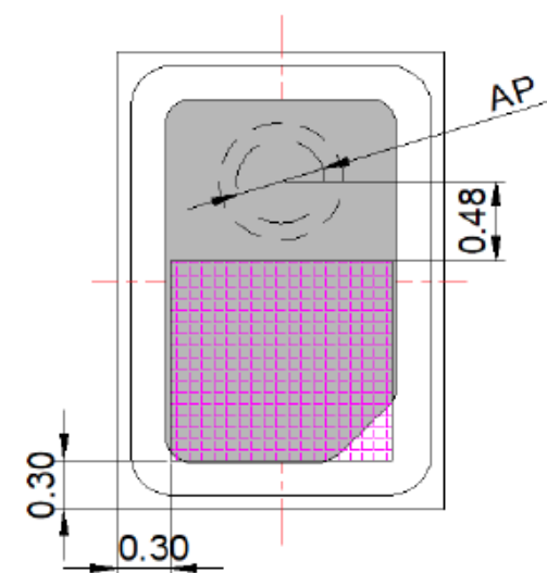
Recommended Pickup Location (Pink area)
