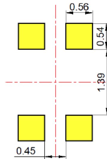
Recommended Solder Pad Layout
