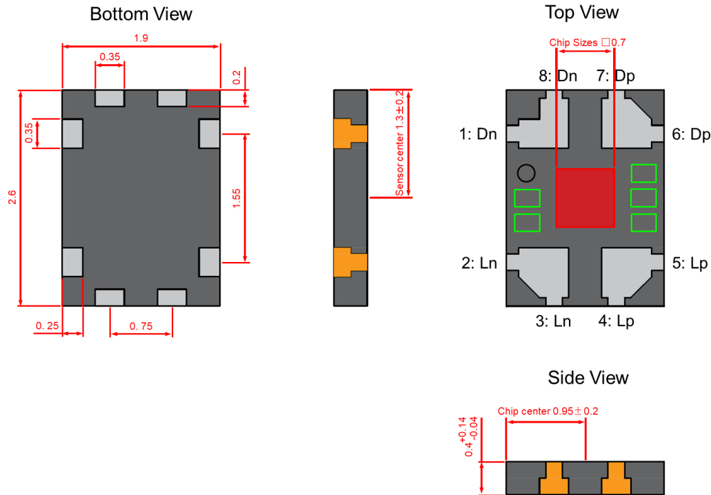
Figure 10.1 Outline Dimensions
