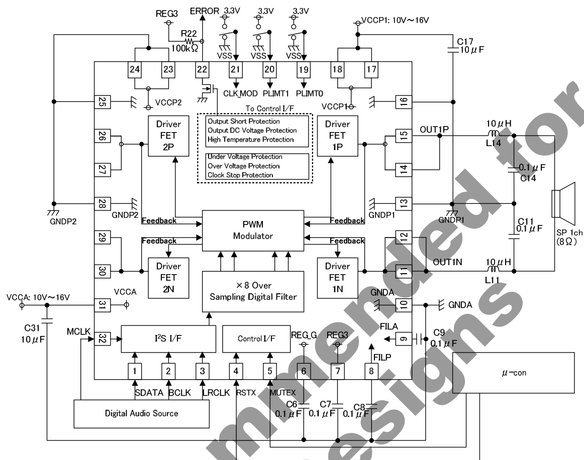
Figure 57. Application Circuit 2
