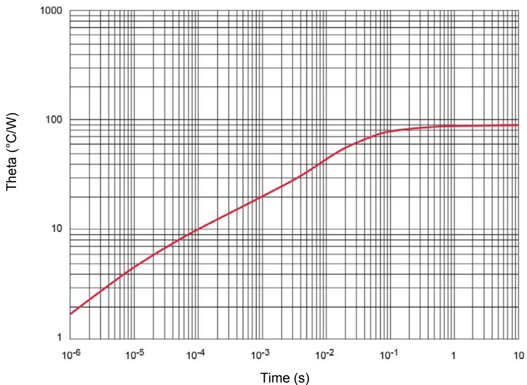
FIGURE 2 Thermal impedance graph ( R_{\theta JSP(IS)} )
