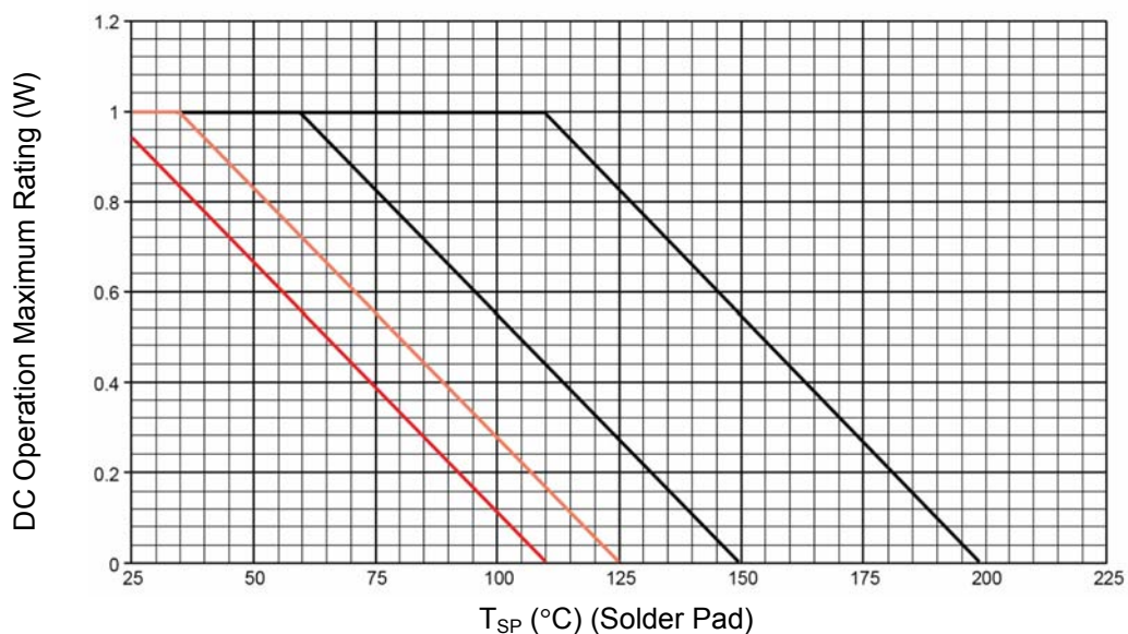
FIGURE 1 Temperature-Power Derating ( R_{\theta JSP(IS)} )
